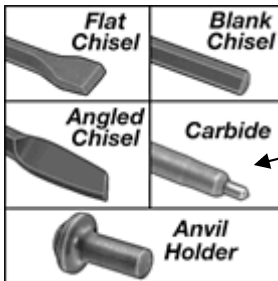
Part 1564T68 Carbide tip estimated cost 21.49.
